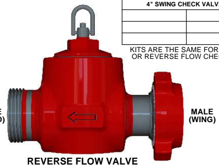
REVERSE FLOW VALVE FEMALE OUTLET ; MALE INLET NOTE THE DIRECTION OF THE ARROW
