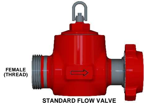
STANDARD FLOW VALVE FEMALE INLET ; MALE OUTLET NOTE THE DIRECTION OF THE ARROW
